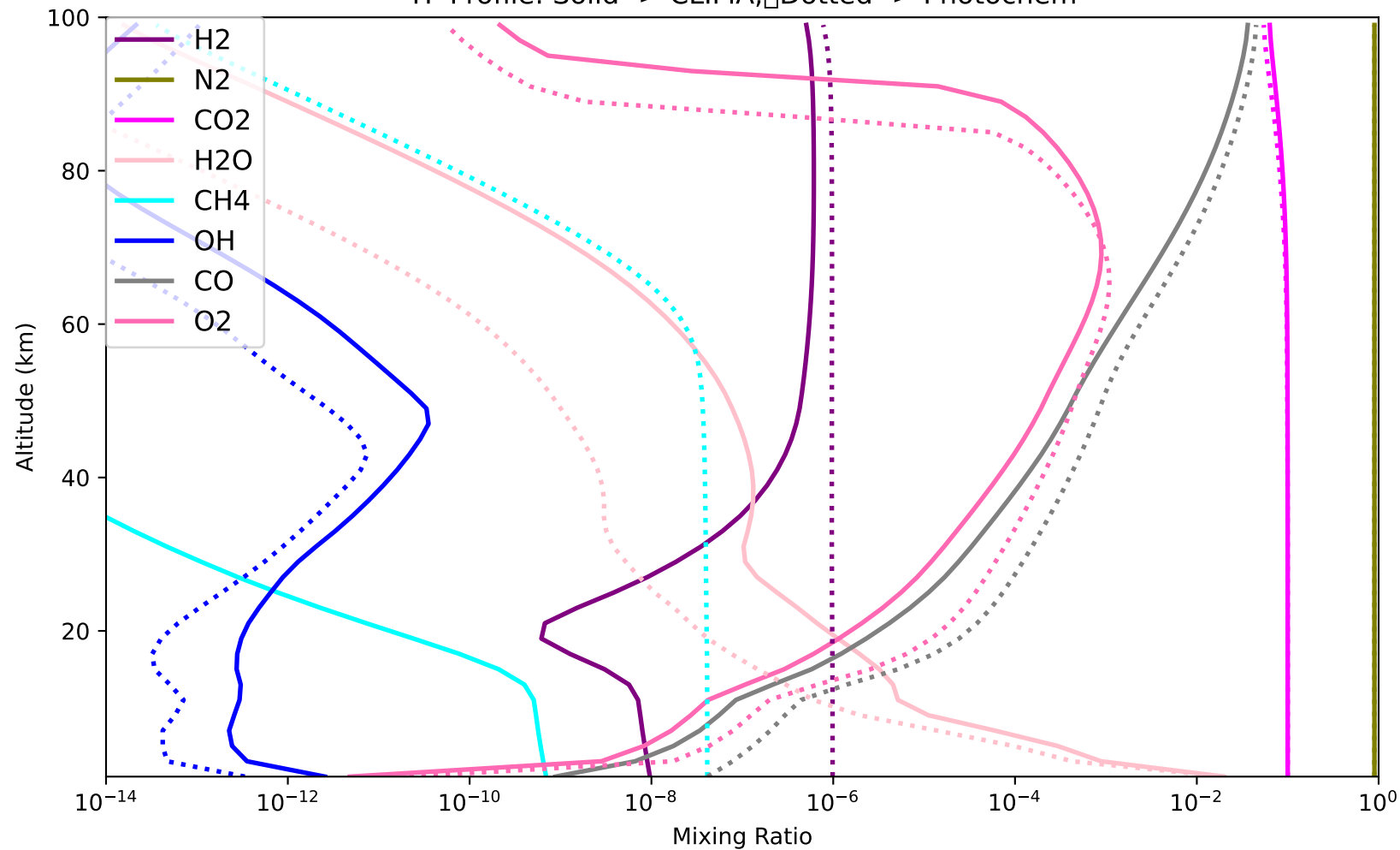
TP Profile: Solid -> CLIMA, Dotted -> Photochem
